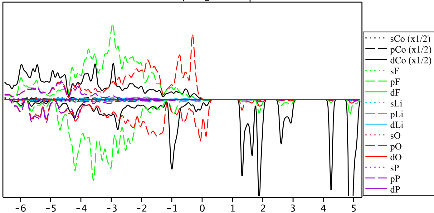
Li2CoPO4F/x50_UGGA-Upaw400
